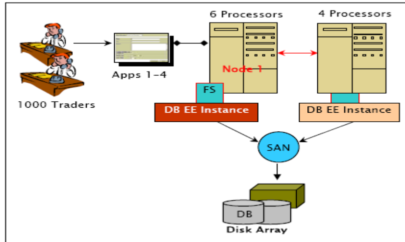
Illustration #4: Failover
